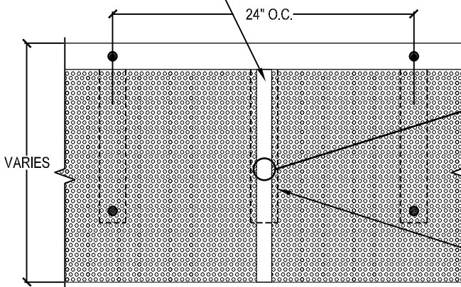
METAL PANEL FRONT VIEW NOT TO SCALE
